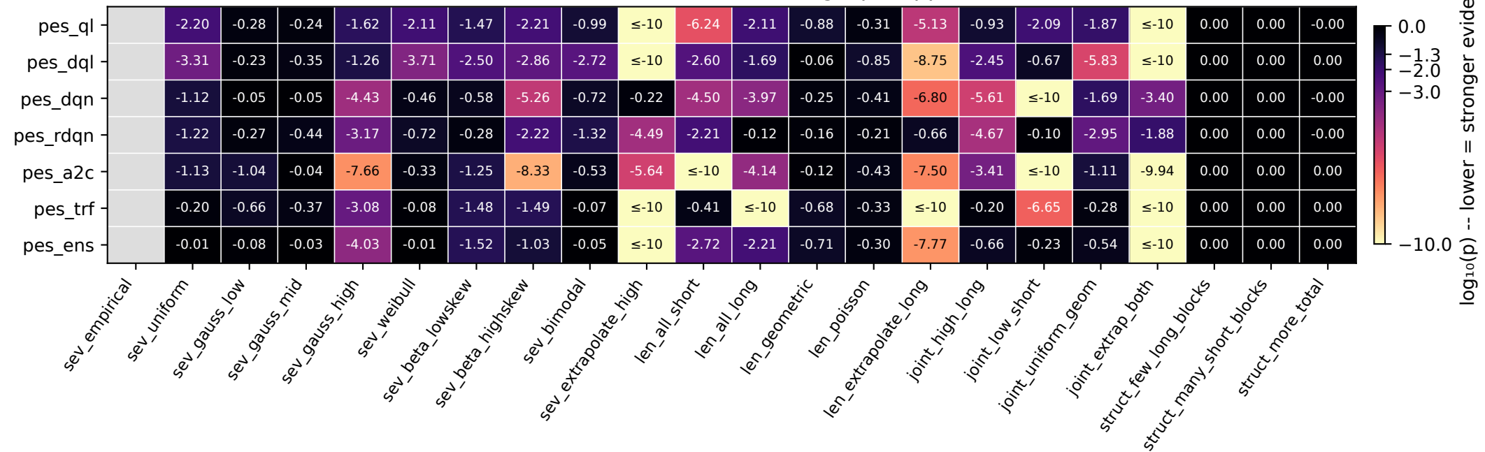
Welch t-test vs in-distribution baseline ( \log_{10} p , clipped to [-10, 0] )
