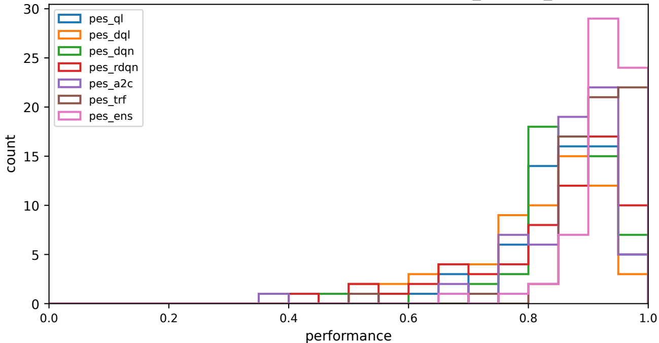
Per-sequence performance distribution -- joint_uniform_geom
