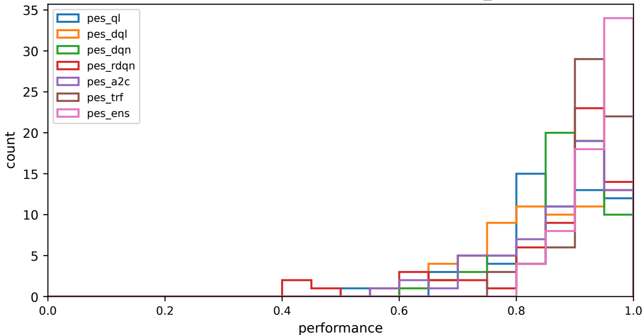
Per-sequence performance distribution -- sev_bimodal
