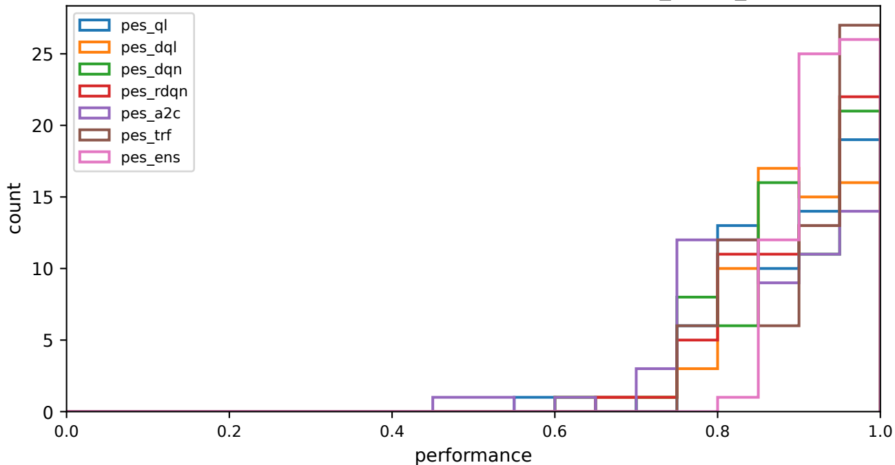
Per-sequence performance distribution -- sev_gauss_low
