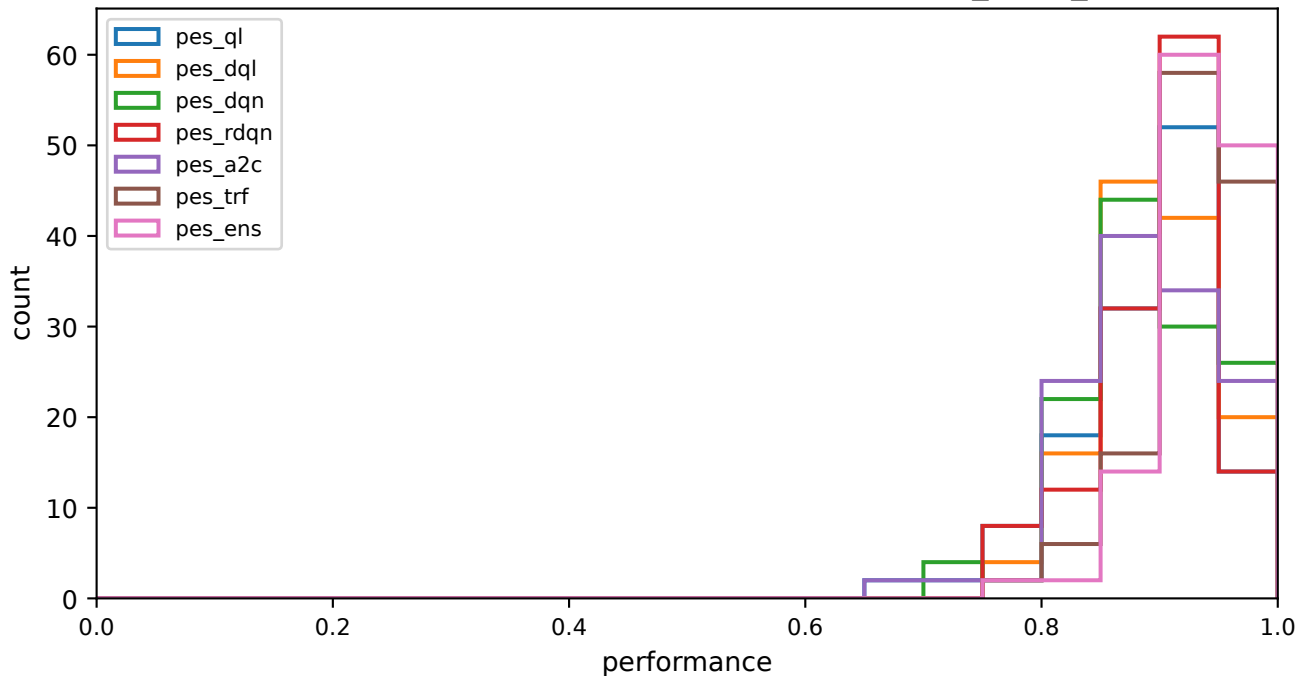
Per-sequence performance distribution -- struct_more_total
