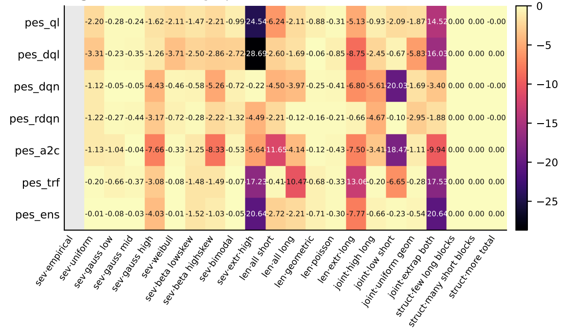
Significancia -\log_{10} p (Welch)
