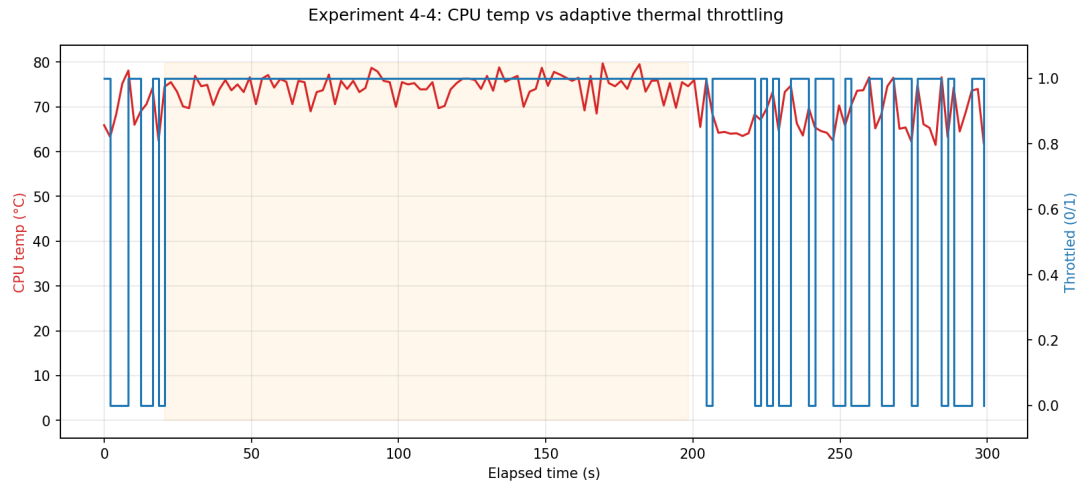
Figure 33: No fan: temperature (red) vs. throttled state (blue) over the full run. The board is continuously throttled through nearly the entire stress window (shaded), then oscillates across the hysteresis band during cooldown as temperature settles near the 65–70 °C boundary.
