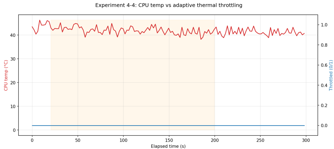
Figure 34: With fan: temperature stays flat in the 38–46 °C range throughout, well clear of the 70 °C trigger — throttling never engages.
