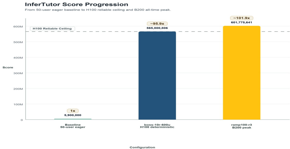
Figure 2. Score progression from 50-user eager baseline (5.9M) to H100 reliable ceiling (565,800,806) and B200 all-time peak (601,775,641). Cumulative multipliers shown above each bar.
