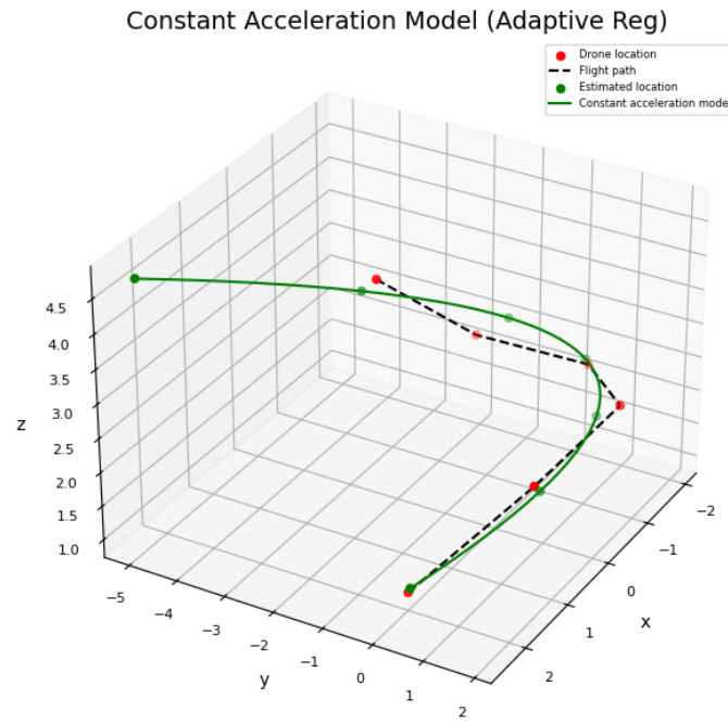
Figure 7: Constant Accelerate Model and the Actual Position (with covariance and angular velocity regression)
