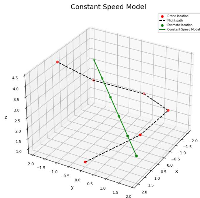
Figure 2: Constant Speed Model and the Actual Position
