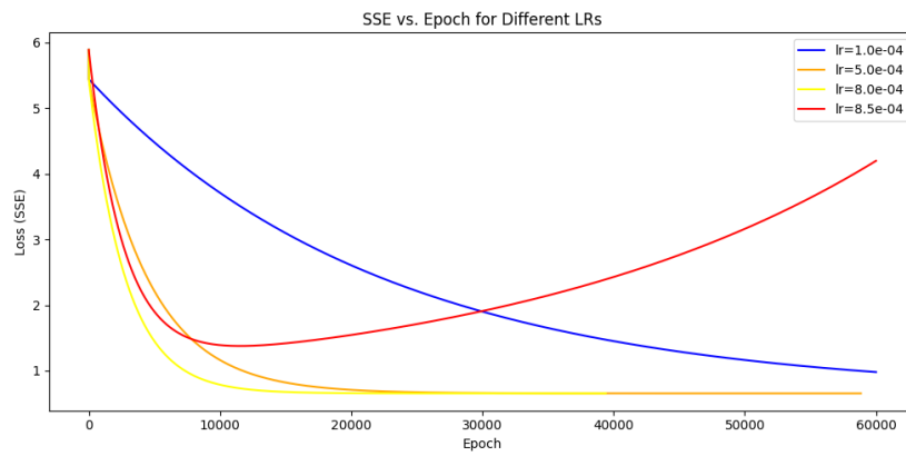
Figure 3: SSE and Epoch for Different LRs
