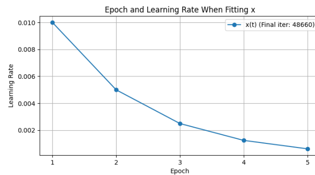
Figure 4: Decaying Learning Rate on x-position Fitting
