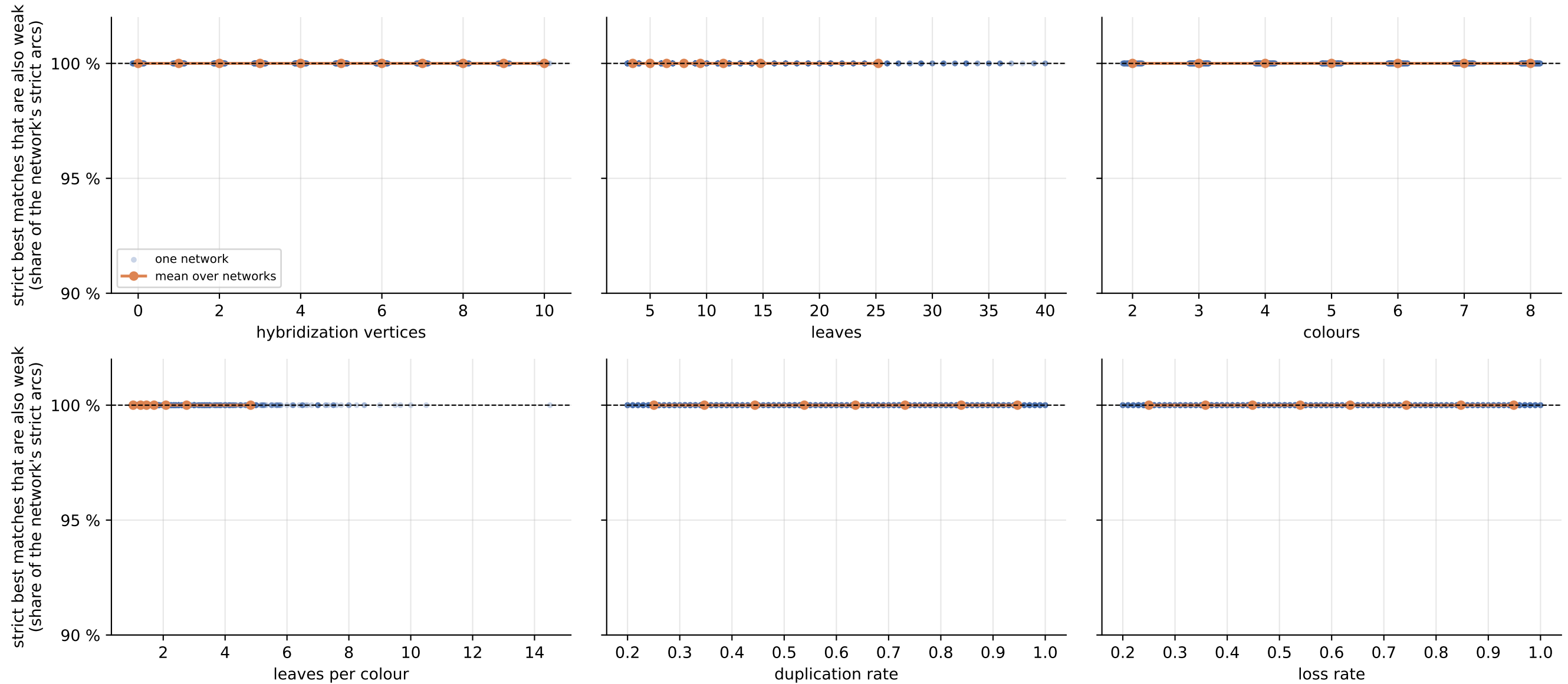
P(weak | strict) per network vs. generator parameters (1800 random networks)
