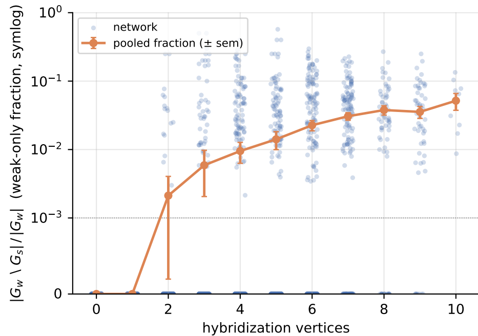
Weak-only fraction vs. generator parameters (1800 random networks; each dot one network; y = 0 shown below dotted line)
