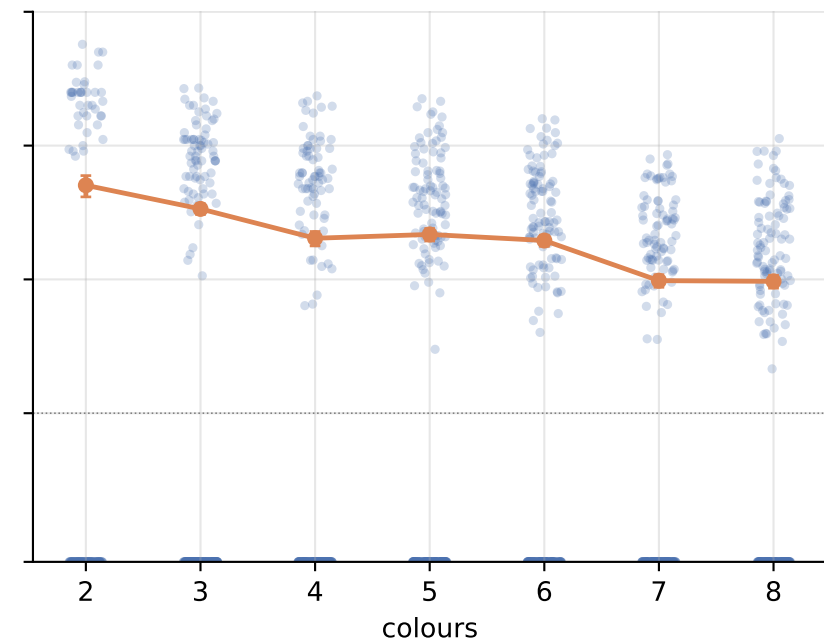
Weak-only fraction vs. generator parameters (1800 random networks; each dot one network; y = 0 shown below dotted line)
