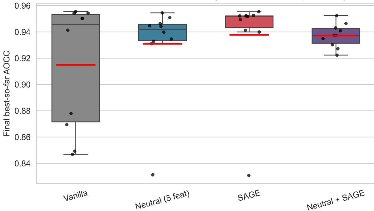
Final AOCC after 500 candidates (10 seeds, H=3.93 , p=0.2692 )
