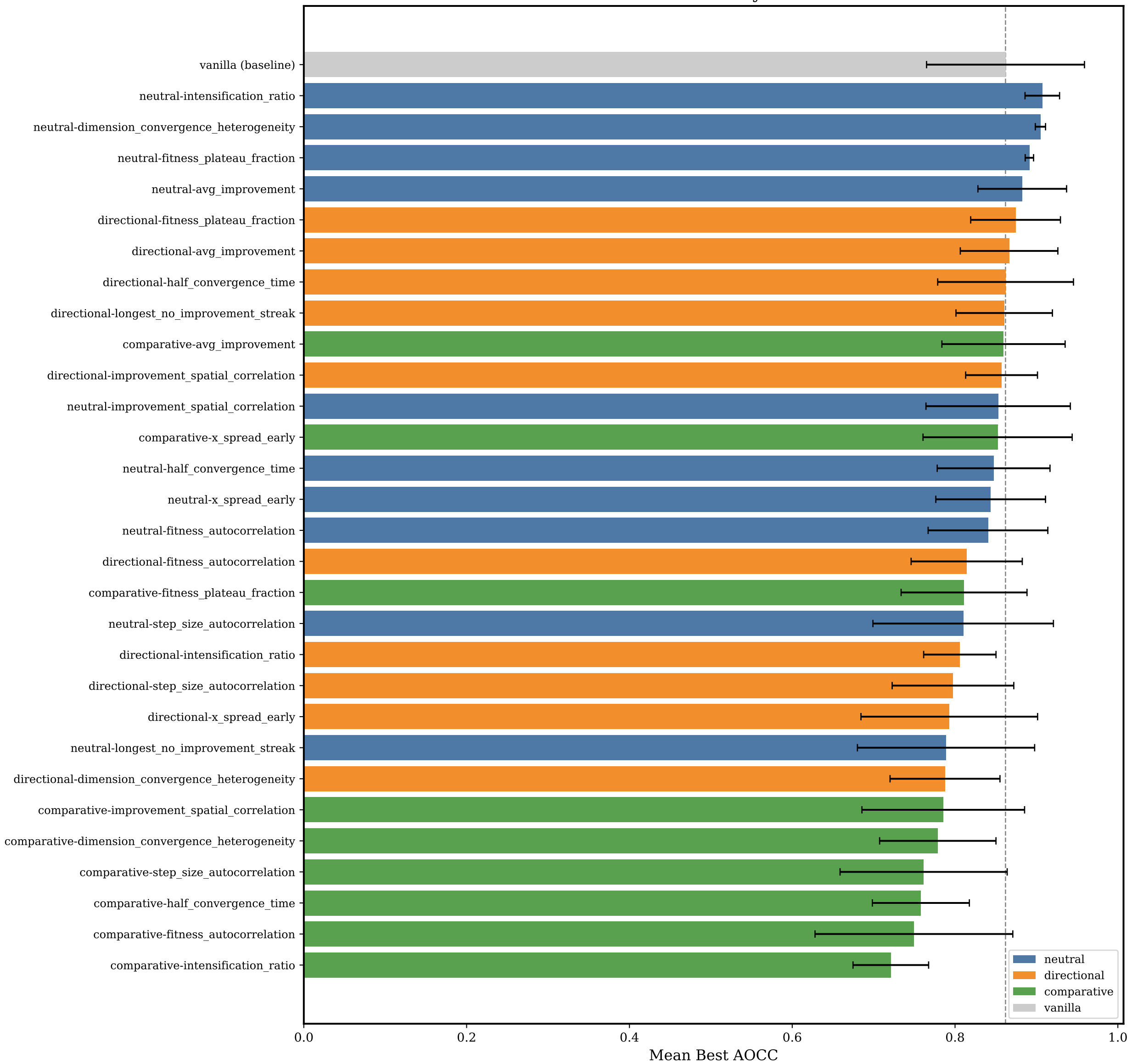
All 29 Conditions Ranked by Mean Best AOCC
