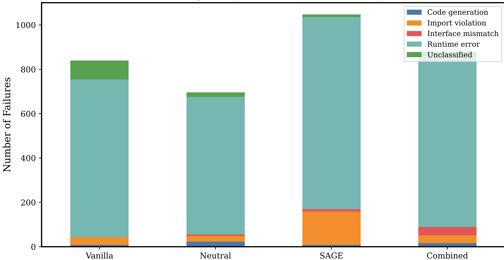
Failure Categories per Condition (all seeds pooled)
