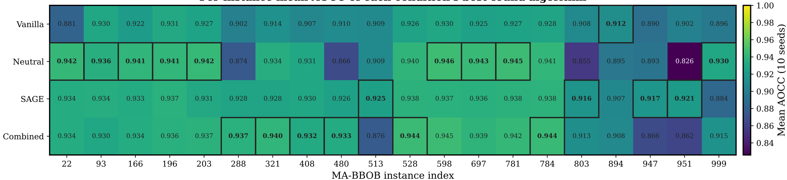
Per-instance mean AOCC of each condition's best-found algorithm
