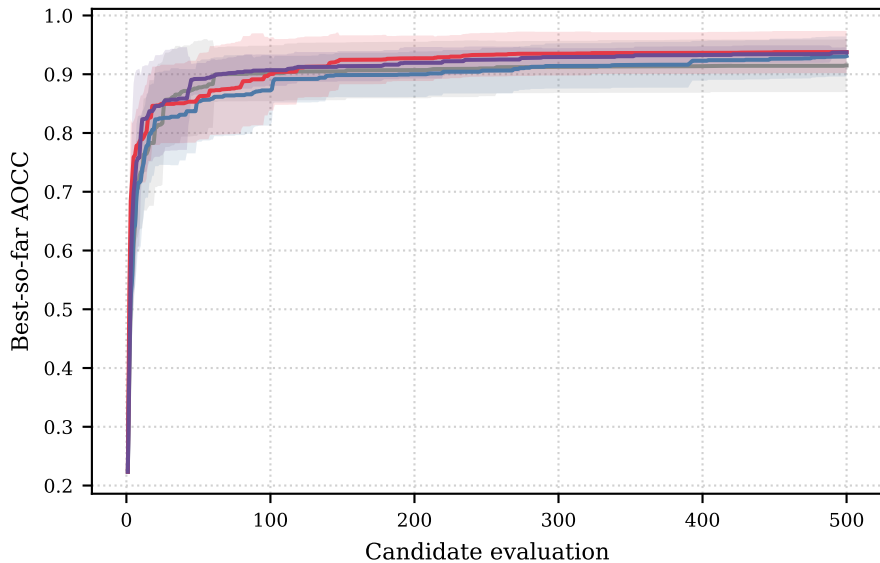
(a) AOCC convergence curve
