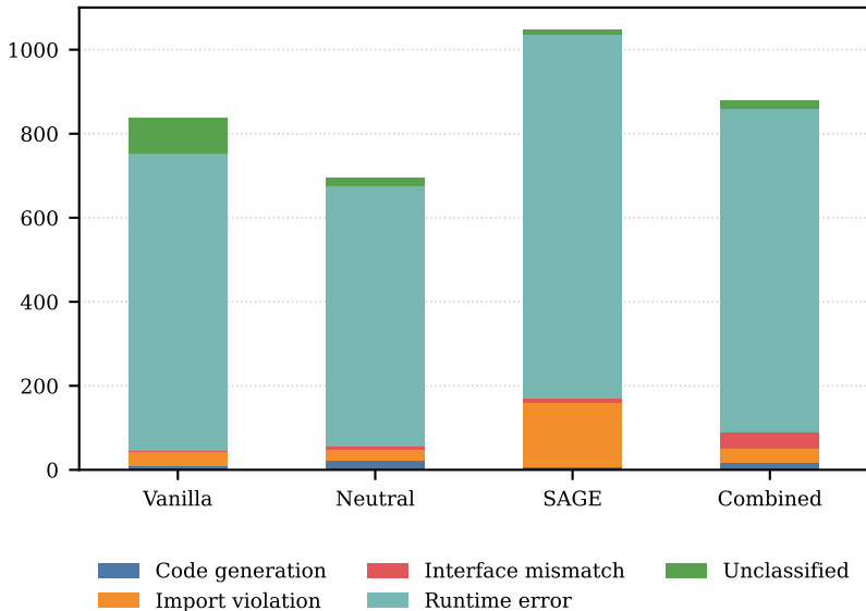
Failure Categories per Condition (all seeds pooled)
