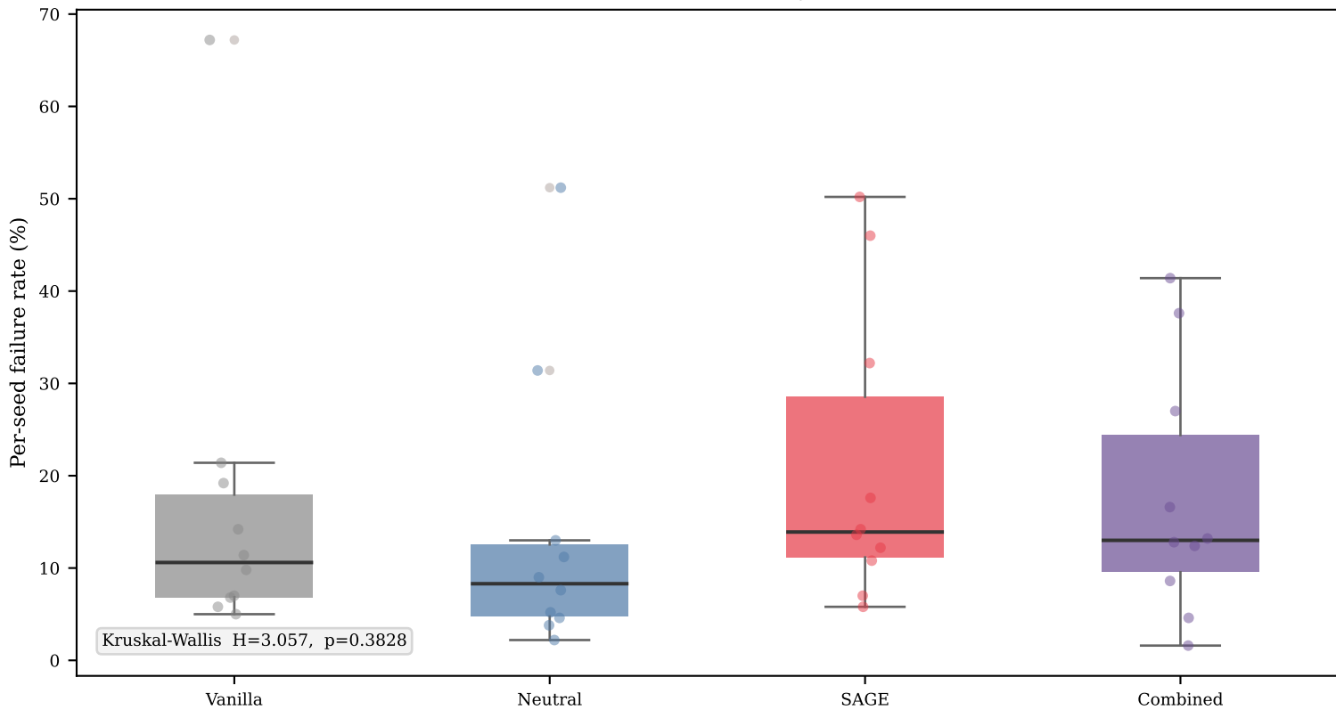
Failure rate distribution by condition
