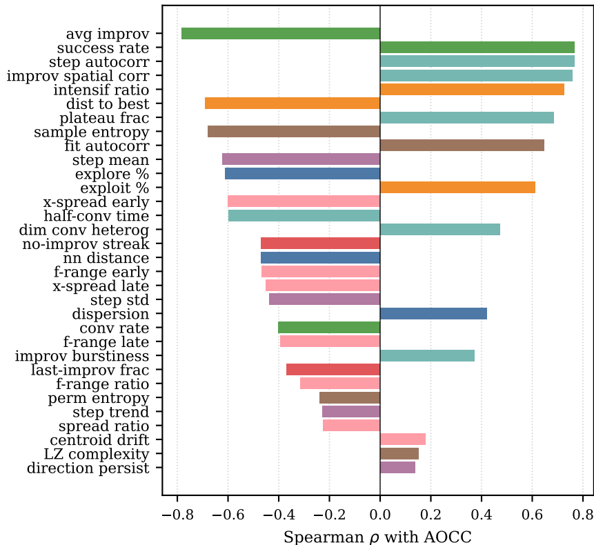
Spearman Correlation with AOCC (Bonferroni-corrected)
