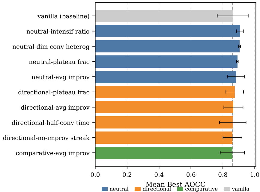
Top 9 Conditions Ranked by Mean Best AOCC
