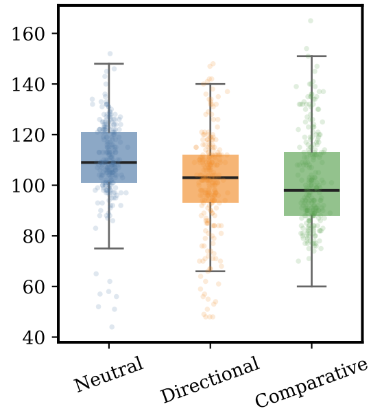
Numeric constants
