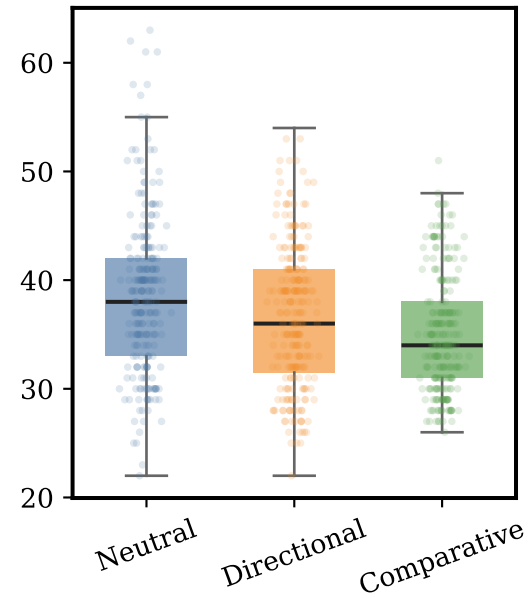
NumPy calls
