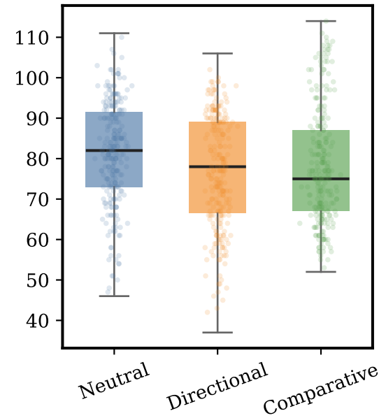
Assignments
