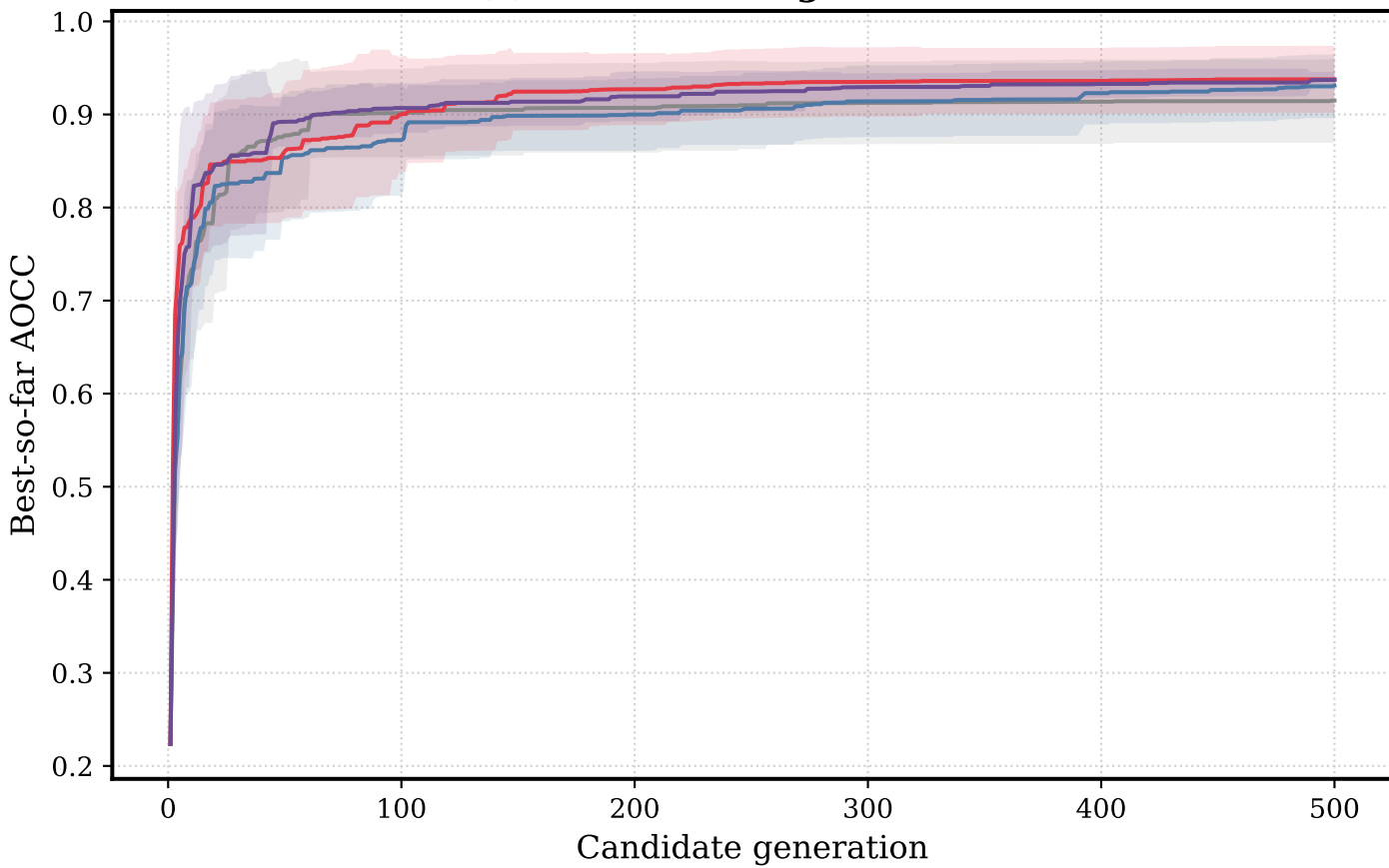
(a) AOCC convergence curve
