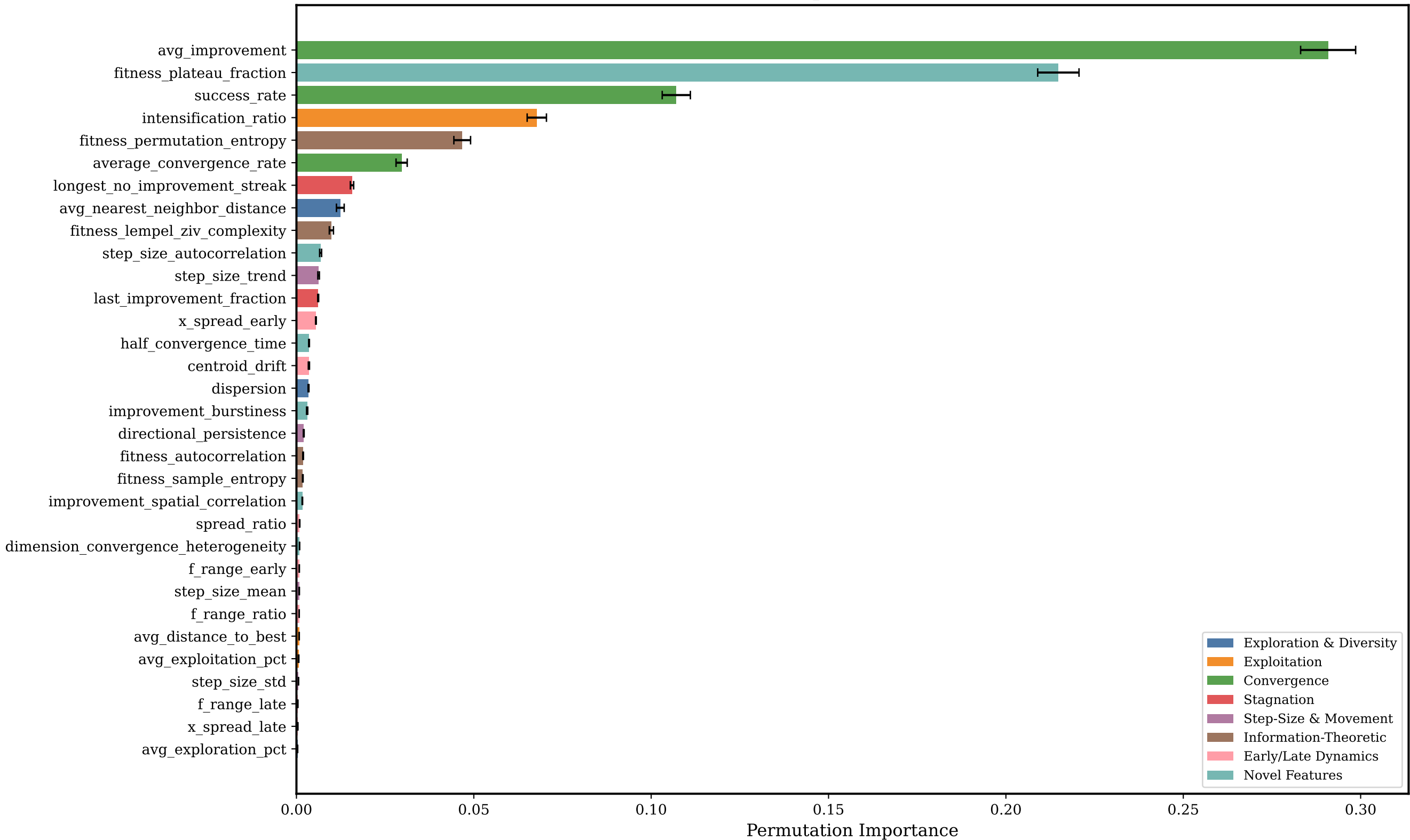
RF Permutation Importance (OOB R^2 = 0.962 )
