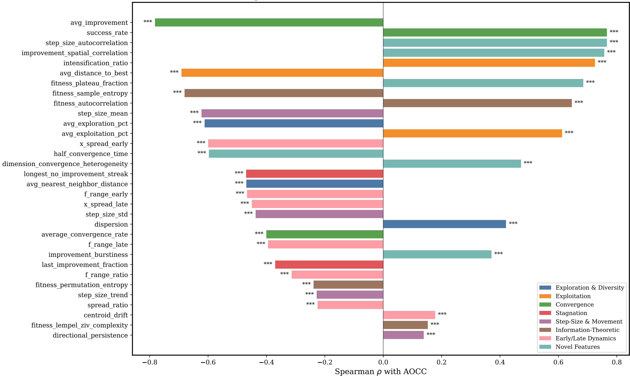
Spearman Correlation with AOCC (Bonferroni-corrected)
