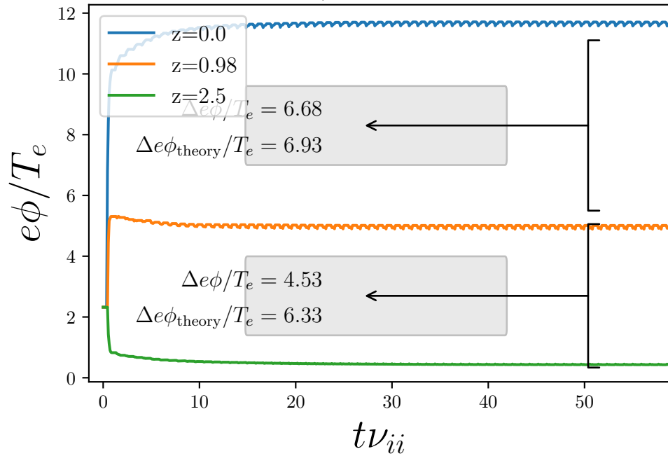
Time trace of \phi at various z locations
