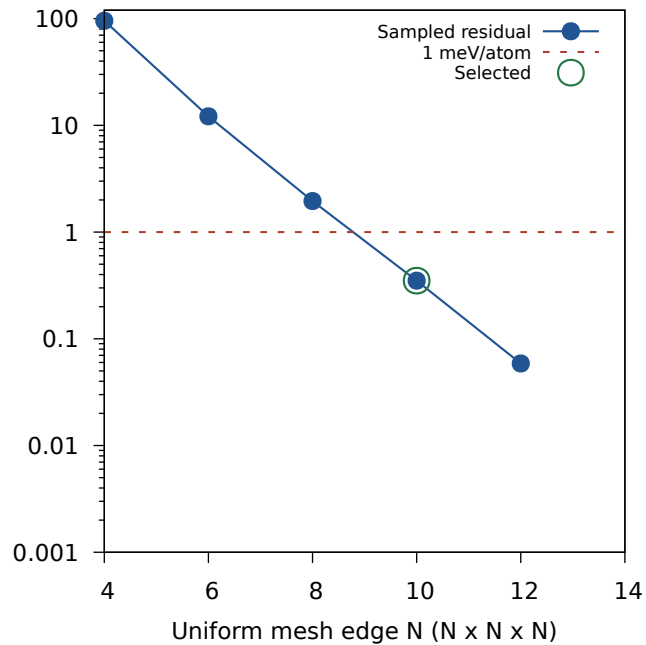
(c) k-mesh
