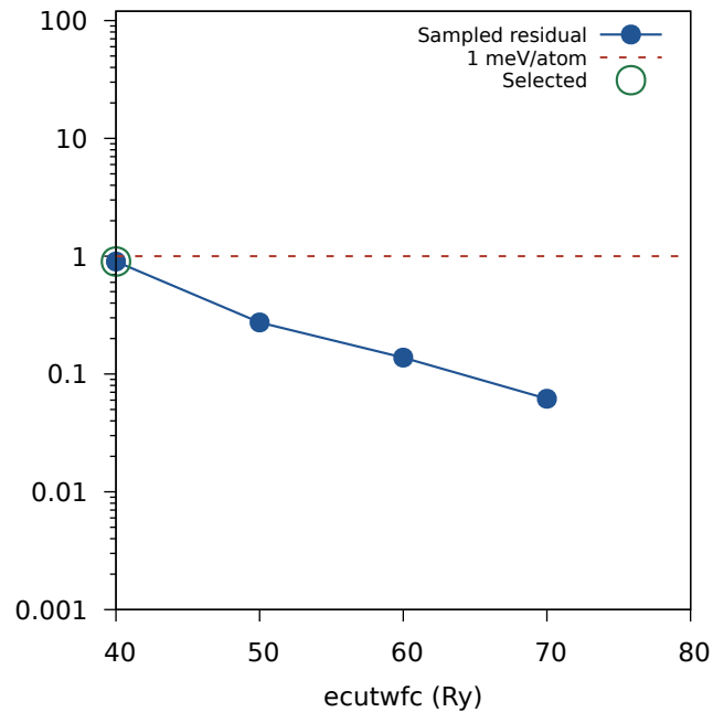
(a) ecutwfc
