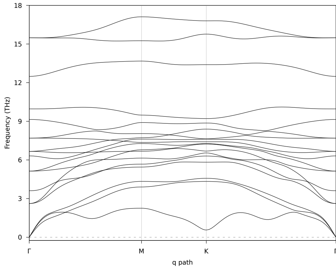
Archived ph64: dispersion
