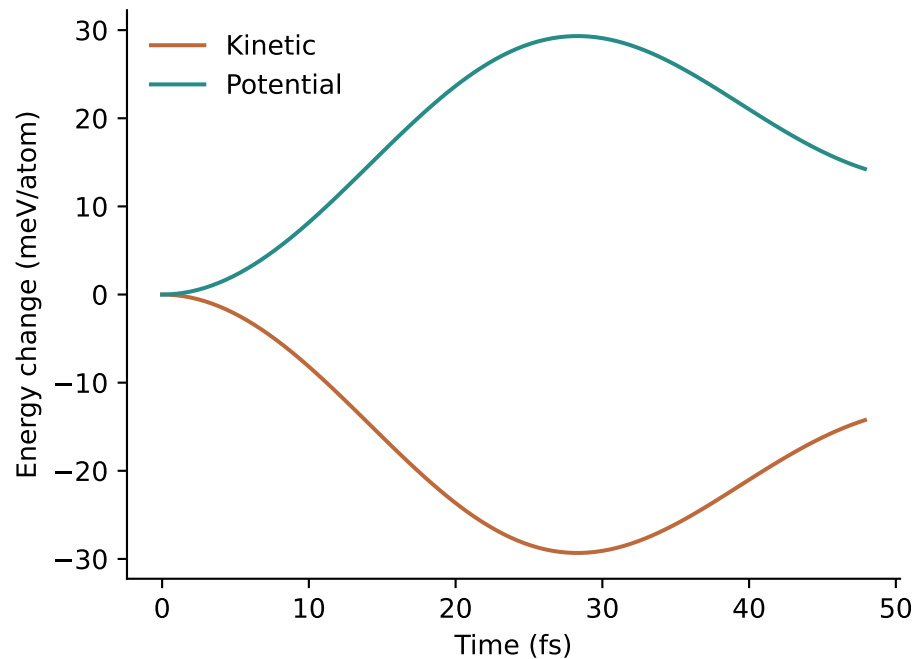
NVE step-size check over ~48 fs | identical initial positions and velocities
