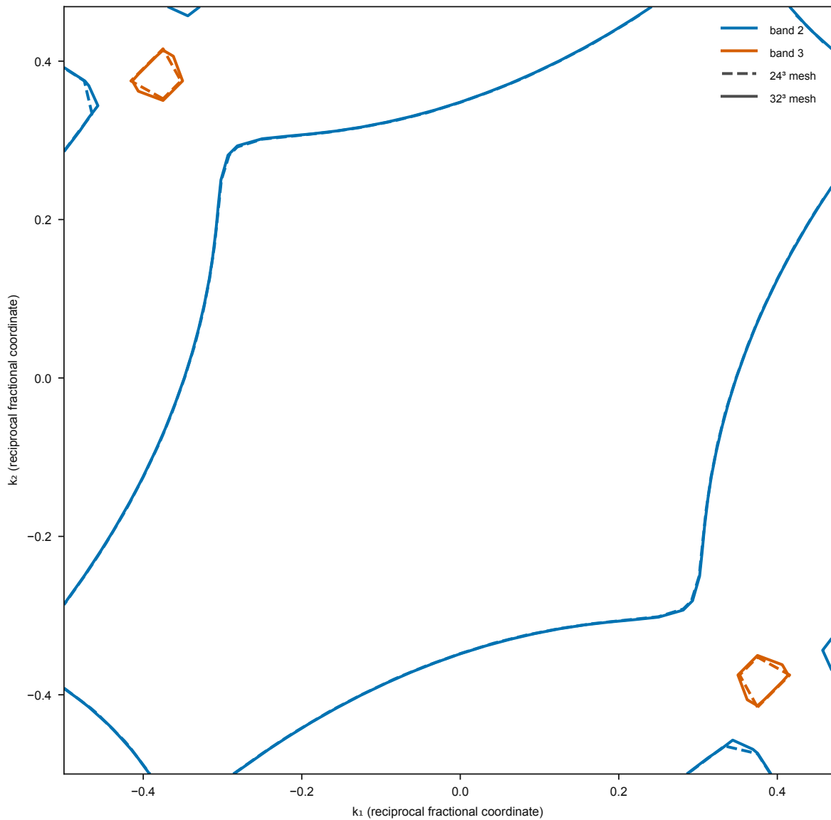
Al Fermi-surface section at k_3=0
