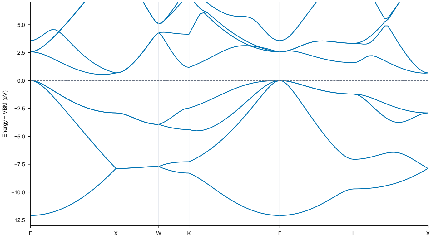
Si, PBE, fixed example cell; no SOC
