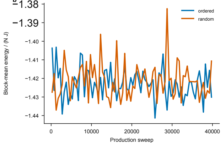
L=24 , T/J=0.92 ; blocks of 500 sweeps
