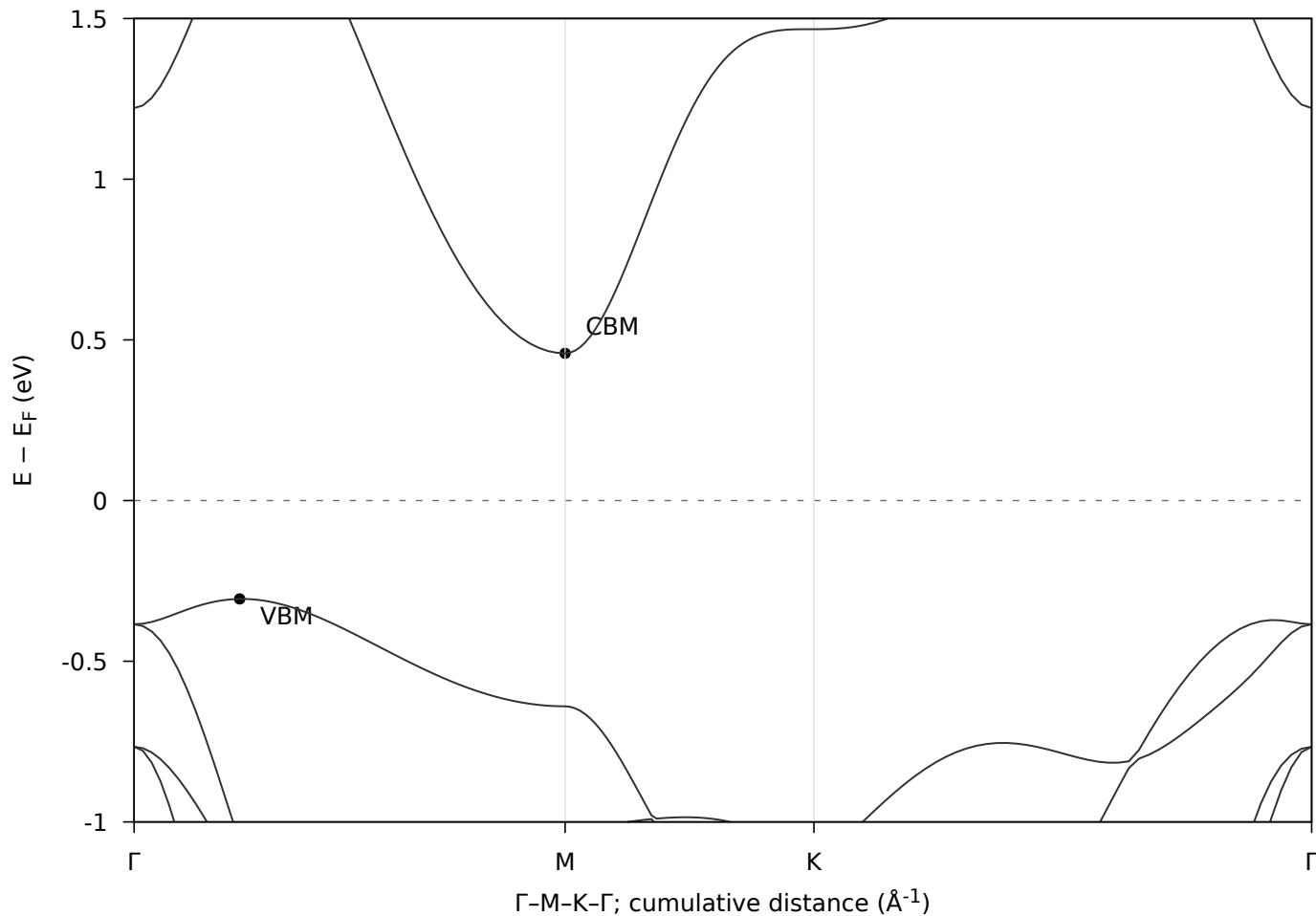
(a) Frozen PBE SnSe 2 : path band edges
