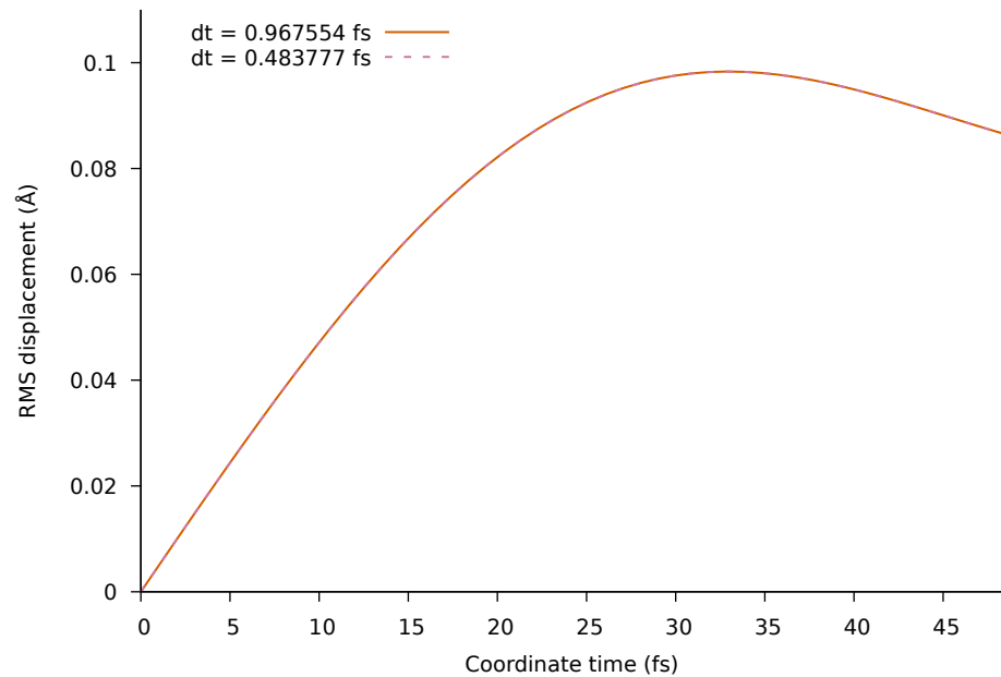
(a) Motion from the shared initial frame
