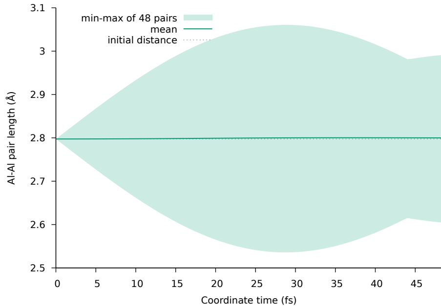
(b) Initial neighbor pairs, fine step
