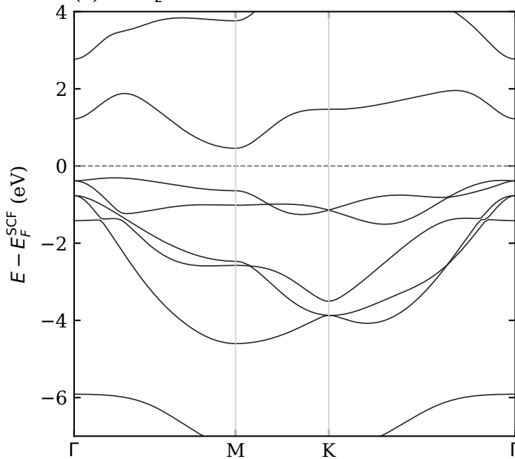
(a) SnSe 2 bands
