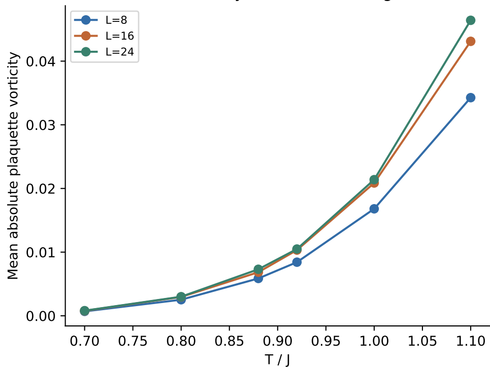
Defect density, not an unbinding test
