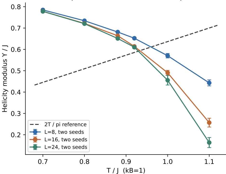
Finite square lattices; no TBKT extrapolation
