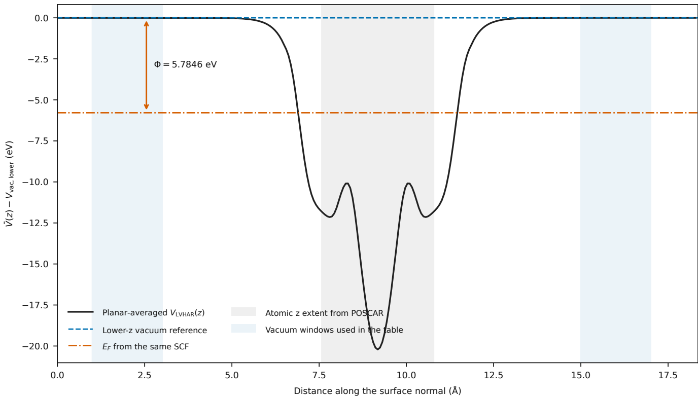
SnSe 2 monolayer: planar-averaged LVHAR and work-function reference
