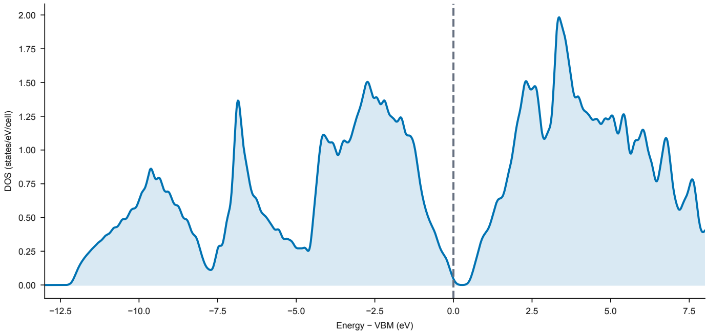
24^3 NSCF mesh; Gaussian broadening 0.01 Ry
