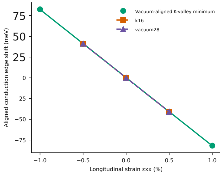
Vacuum-aligned K edge
