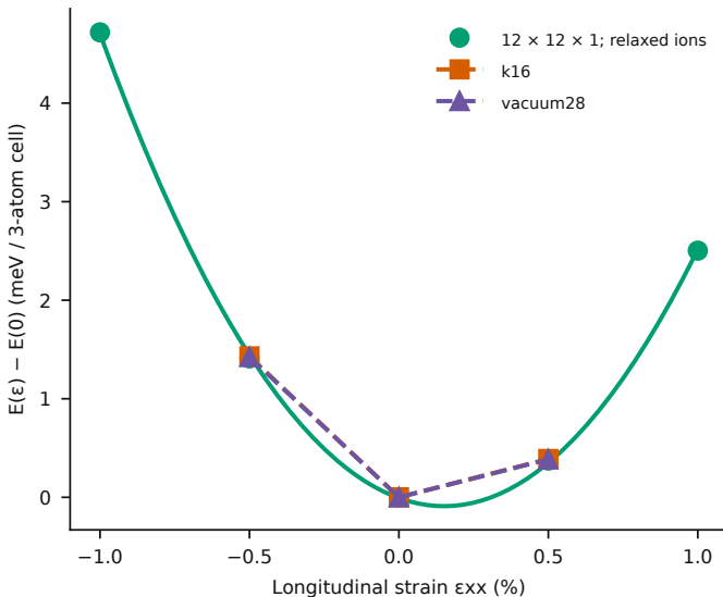
Strain energy
