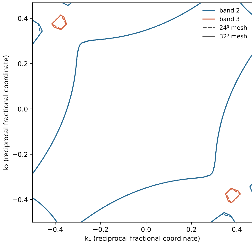
Al Fermi-surface section at k_3=0
