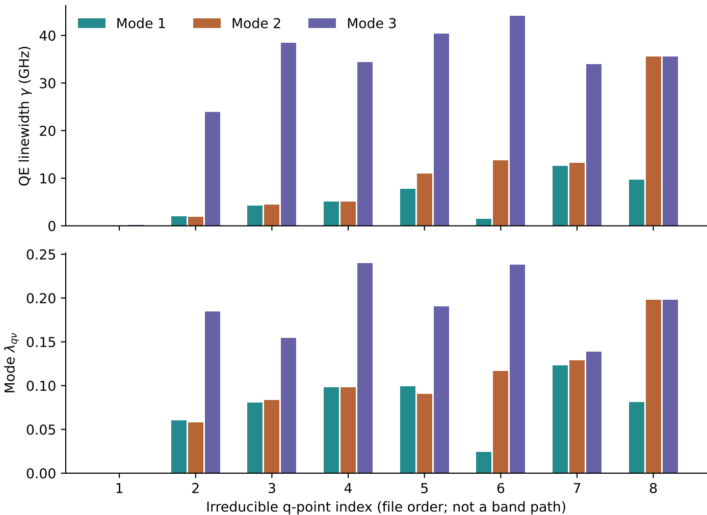
fcc Al | electronic width 0.020 Ry Raw ph.x values; \Gamma acoustic residual is not an optical mode
