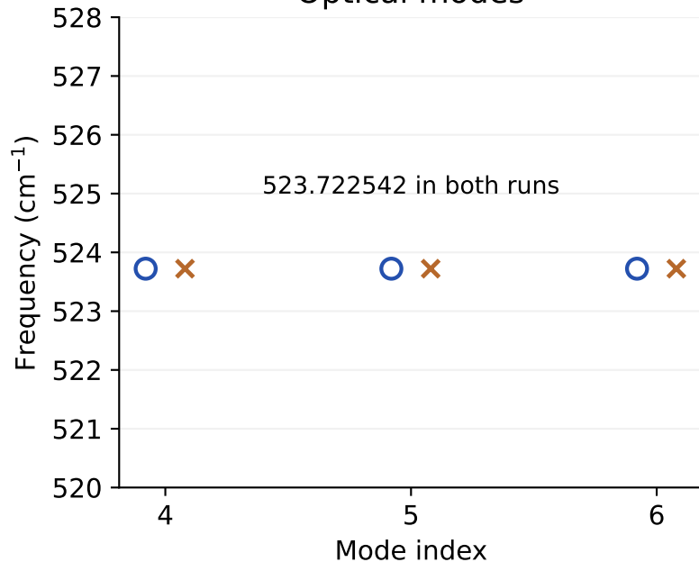
Optical modes
