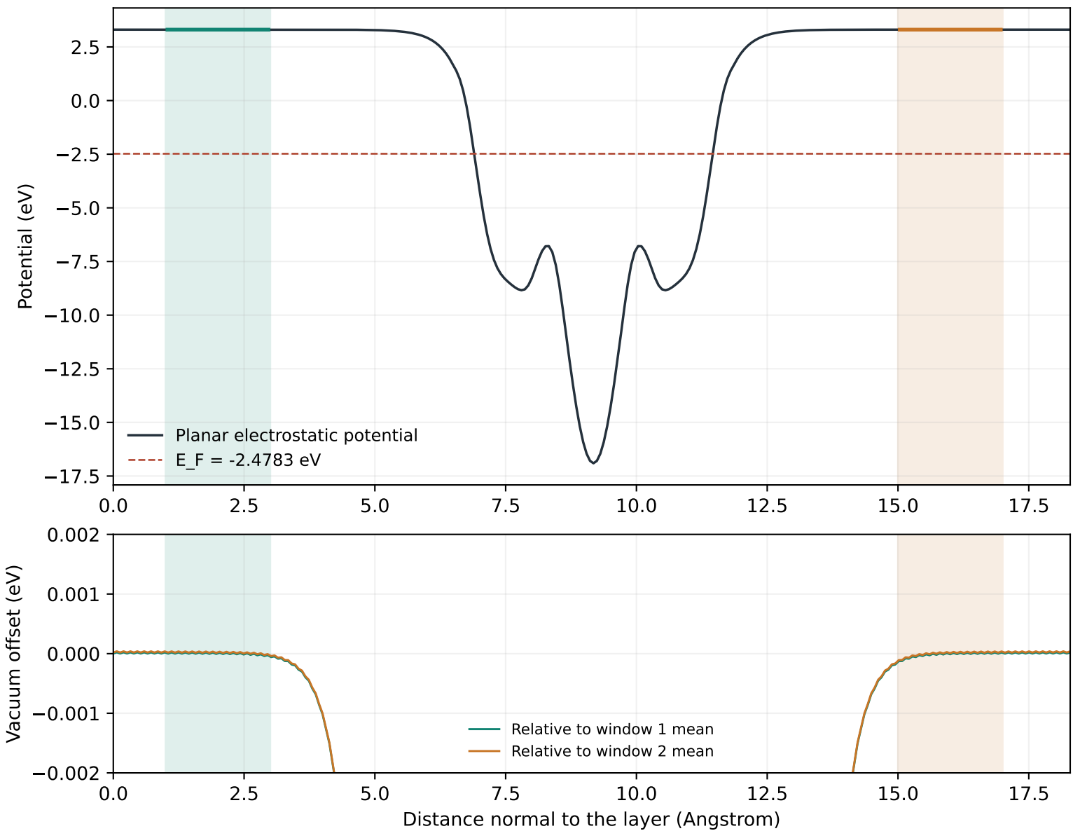
SnSe2: self-consistent 33 x 33 x 1 mesh, LVHAR
