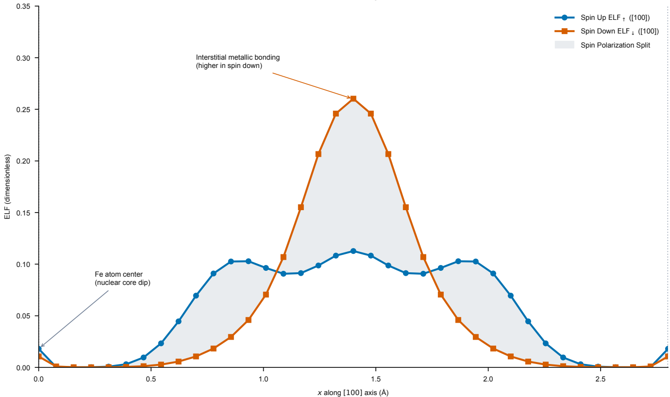
bcc Fe: 1D ELF Linecut along [100] Direction
