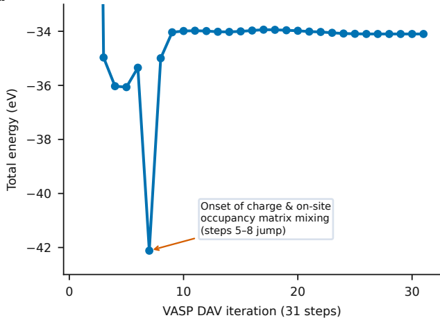
VGe 2 P 4 DFT+ U ( U_{\text{eff}} = 3.0 eV) convergence
