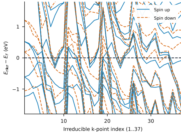
Spin-polarized Kohn-Sham states (mag = 0.578 \mu_B )
