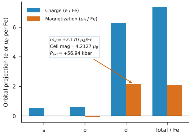
Spin-resolved Fe-3d moment & stress check
