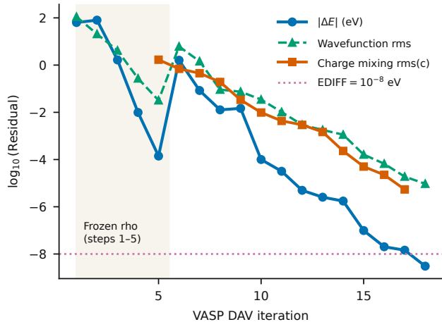
bcc Fe SCF convergence (NELMDL = -5)
