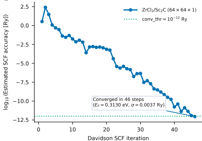
2D metallic heterostructure (charge sloshing)
