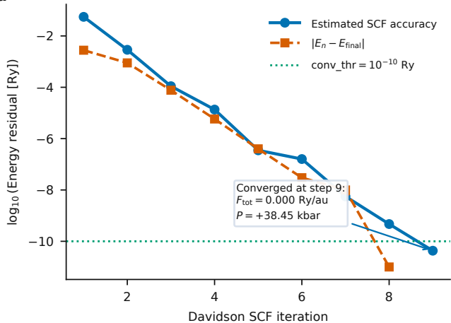
Gapped Si ( 8 \times 8 \times 8 , monotonic)
