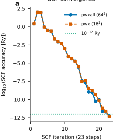
SCF convergence
