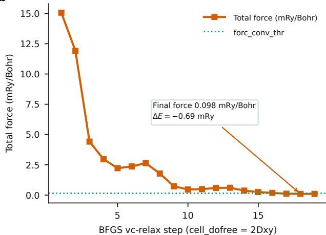
\text{ZrCl}_2/\text{Sc}_2\text{C} 2D in-plane vc-relax
