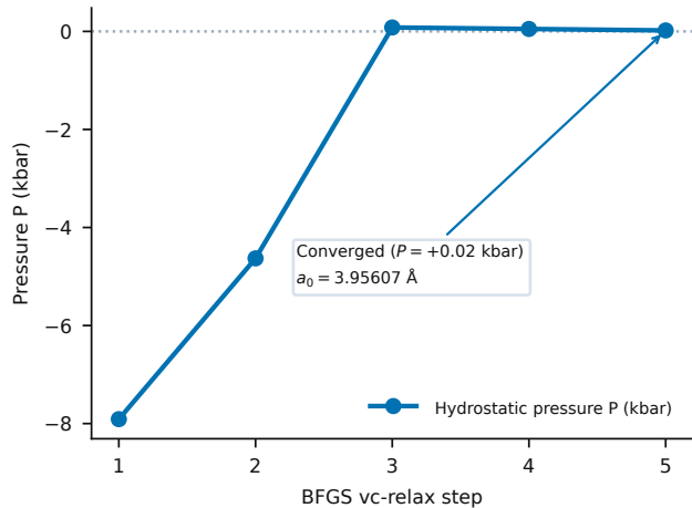
fcc Al 3D vc-relax convergence
