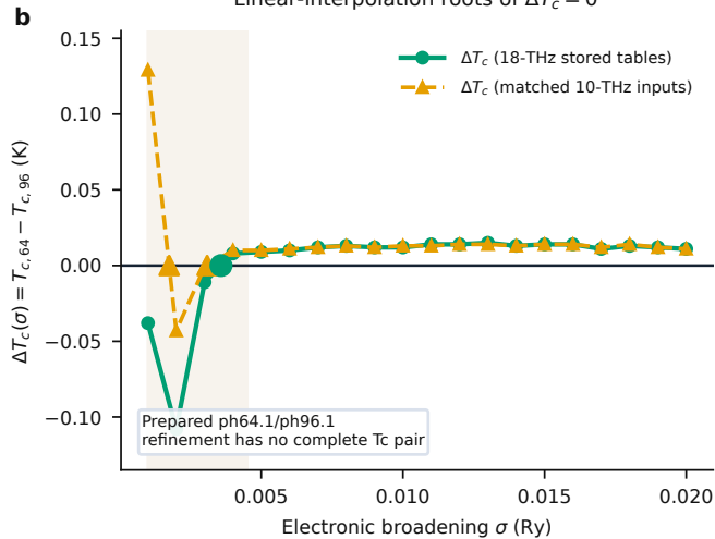
Linear-interpolation roots of \Delta T_c = 0
